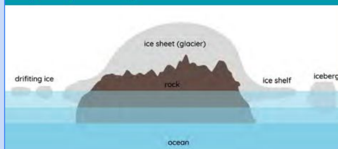
Physical features of Antarctica
